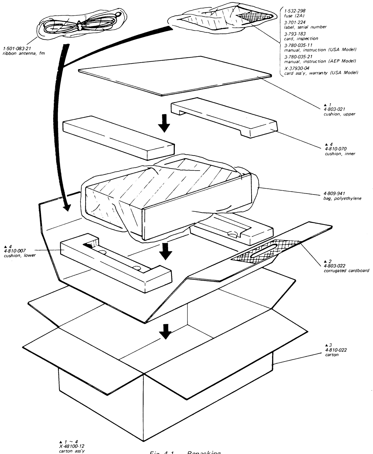
Fig. 4-1. Repacking
