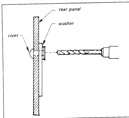
Fig. 2-20. Rivet removal
