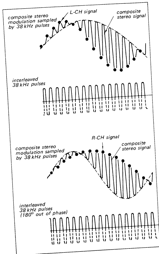
Fig. 1-1. Stereo demodulation operation
